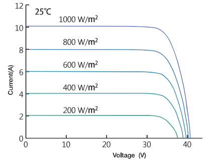
Current-Voltage Curve under different irradiance
